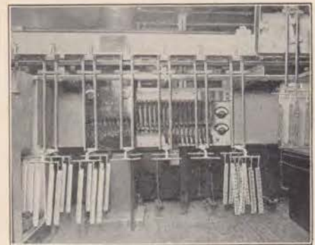
Parts to be electro-galvanized are loaded on racks, which carry them automatically through the various cleaning solutions, and the electrolyte. Operators load the racks and unload the plated parts; the machine does the rest.
