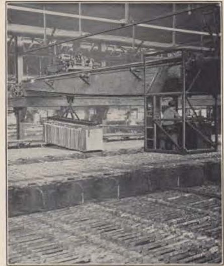
In the electrolytic process the anode is made of the metal to be purified. The electrolyte is a copper sulphate solution containing free sulphuric acid and, usually, a small amount of common salt or some other soluble chloride. The current travels through the solution, carrying copper from the anode and depositing it on the cathode plate. The deposited metal is about 99.93 per cent pure copper.
