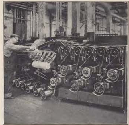
A "steam wipe" tinning machine, which puts a thin coat of tin on copper wire before it is insulated to facilitate soldering to other wire or to apparatus.
