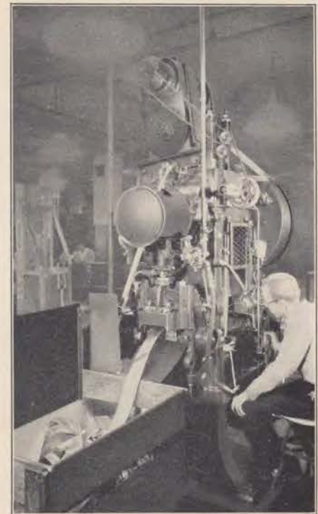
Tens of thousands of springs containing nickel are used in making telephone equipment. Machines like this punch springs out of long strips of metal.
