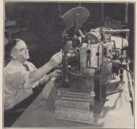
This machine performs the operations of sealing and exhausting the glass bulbs of switchboard lamps. These lamps employ very small drawn tungsten wire (.004 of an inch in diameter) as filament material.
