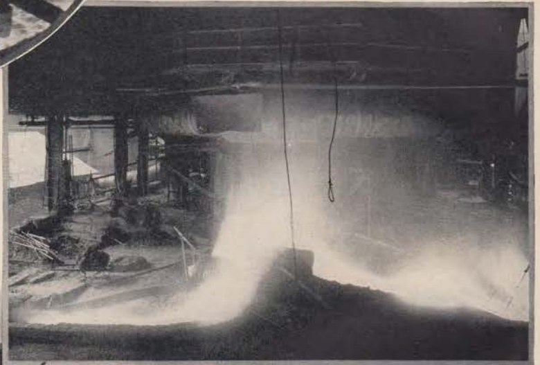
The tapping floor of a blast furnace, showing molten iron issuing from the furnace. Molten slag, being lighter than iron, floats on the top and is skimmed off, going down the trough at the right into a slag car. The molten iron flows off to the left into a hot-metal car.
