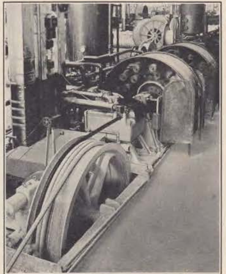
Tape armoring machine showing jute serving heads and application of whiting to the armored cable on the take-up capstan.
