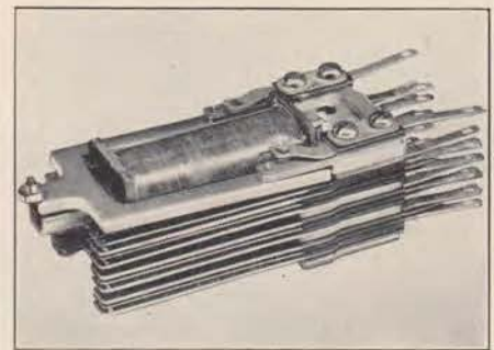
Nickel is part of the alloy used in the relay illustrated above, a type employed by the tens of thousands in telephone systems. Nickel is used in the winding wire, contact springs, magnetic structure and finish of the relay.
