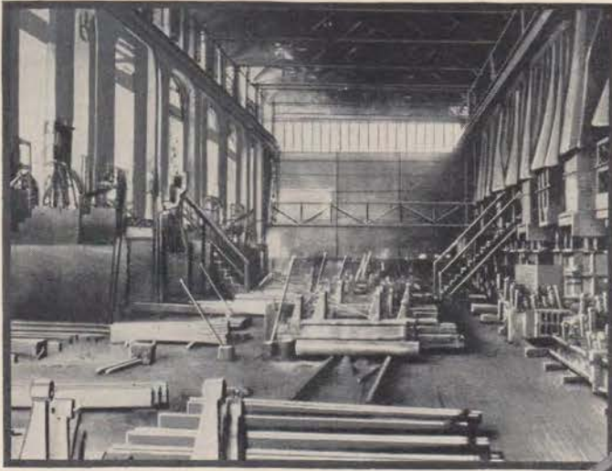
Left—Molding floor of a brass foundry with spare molds on the floor and electric furnaces on the right.
