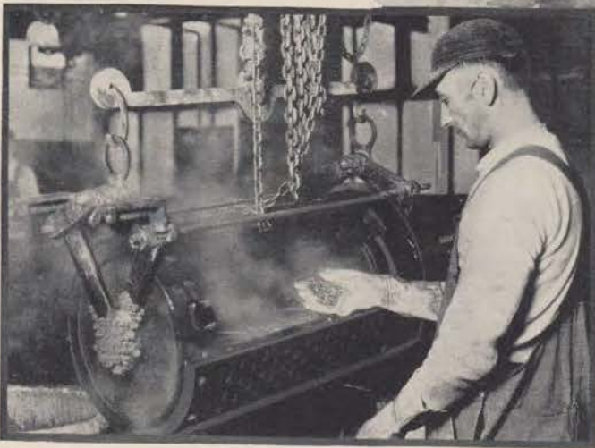
Below—Galvanizing, a process that protects iron from moisture and rust, is done by immersing the parts in molten zinc or by applying the zinc electrolytically.
