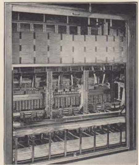
Copper wire by the mile is used in switchboards. This copper wire brings voices to the operator, completes voice pathways between talking subscribers, permits current to pass around iron bars to form magnets and leads current to lamps which flash signals on and off.
