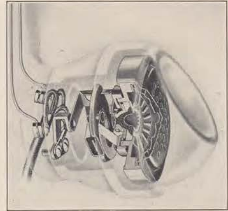
A phantom view of your handset transmitter. The dome-shaped dark mass in the center is the carbon granules. There is a paper seal between the diaphragm and the electrode to prevent the carbon granules from leaking out.
